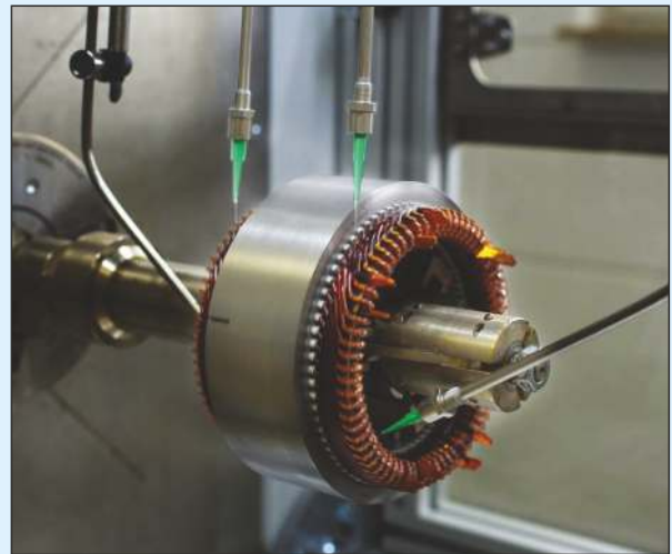
Trickle impregnating of armature
